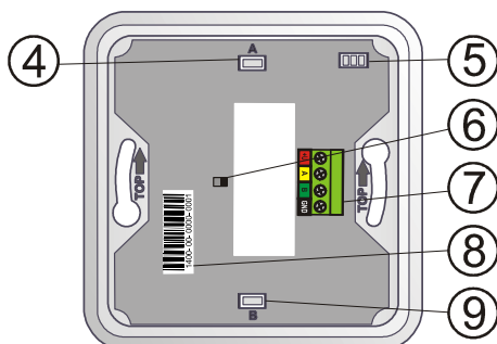
Figure 2: 4 – A button, 5 – LED indicator, 6 – Tamper contact, 7 – BUS terminals, 8 – Production code, 9 – B button
