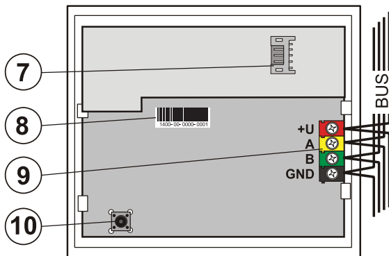
Figure: 7 – control segment connector; 8 – production code; 9 – bus terminals; 10 – tamper contact
