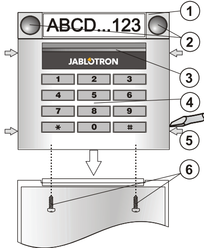
Figure: 1 – control segment; 2 – segment buttons; 3 – backlit activation button; 4 – keypad module with RFID reader; 5 – tabs for opening; 6 – cover screws
