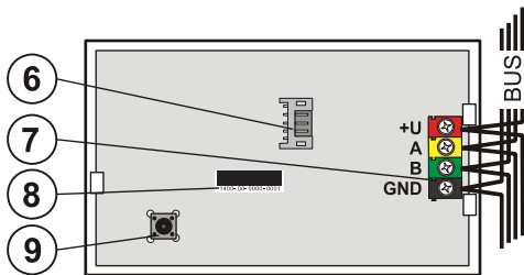
Figure: 6 – control segment connector; 8 –, 7 – bus terminals, 8 – production code; 9 – tamper contact
