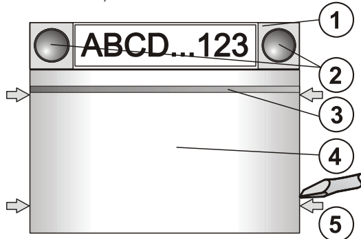
Figure: 1 – control segment; 2 – segment buttons; 3 – backlit activation button; 4 – RFID module; 5 – tabs for module opening
