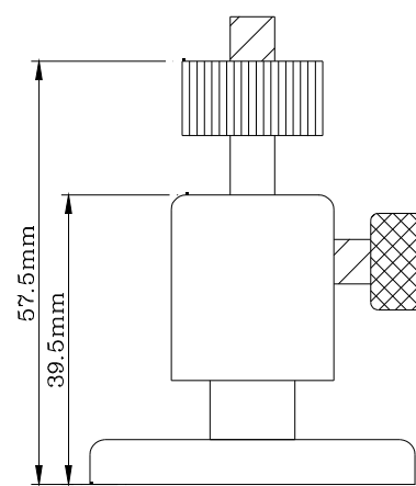
Mounting Bracket
